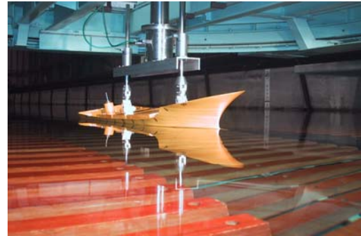
Fig.4 Setup of the captive model experiment.
