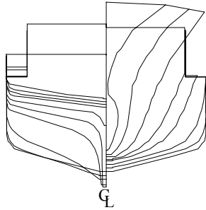
Fig.1 Body plan of the subject ship
